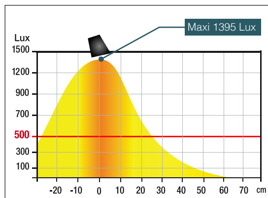
Measurement of Lux on the worktop with a 27 cm profile:
