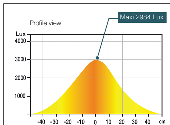
LUX measurement upwards at 55 cm from the light source:
