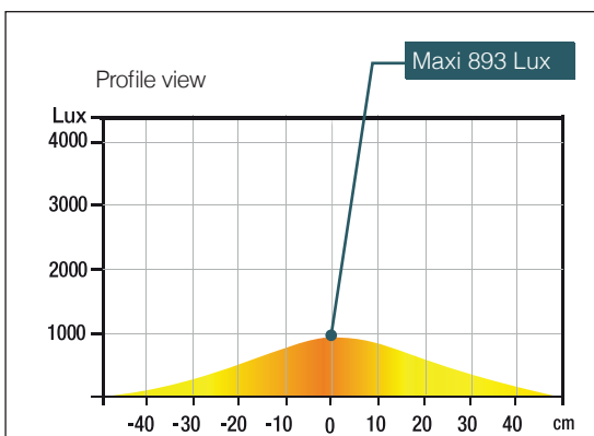
Measurement of Lux down to 110 cm from the light source:
