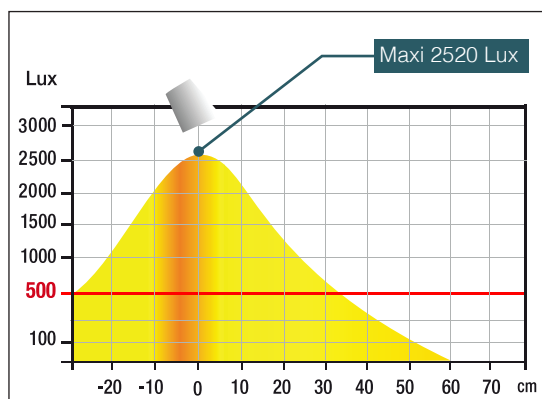
Measurement of LUux on the worktop with a 35 cm profile:
