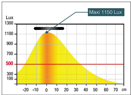
Measurement of Lux on the worktop with a 40 cm profile:
