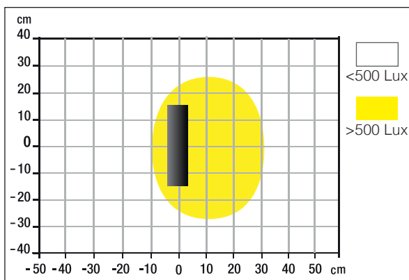
Measurement of Lux on the worktop in 40 cm top view:
