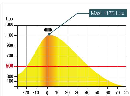
Measurement of Lux on the worktop with a 50 cm profile:
